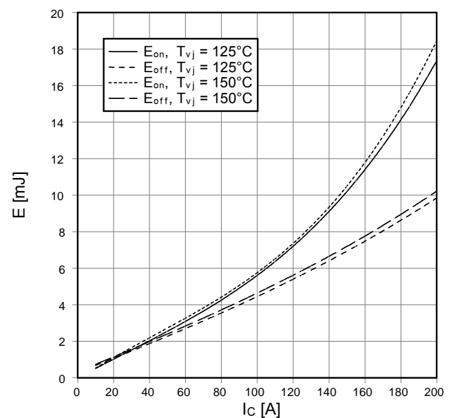
Schaltverluste IGBT-Wechselr. (typisch) switching losses IGBT-inverter (typical) E_{on} = f(I_C) , E_{off} = f(I_C) V_{GE} = \pm 15\text{ V} , R_{Gon} = 24\ \Omega , R_{Goff} = 24\ \Omega , V_{CE} = 300\text{ V}
